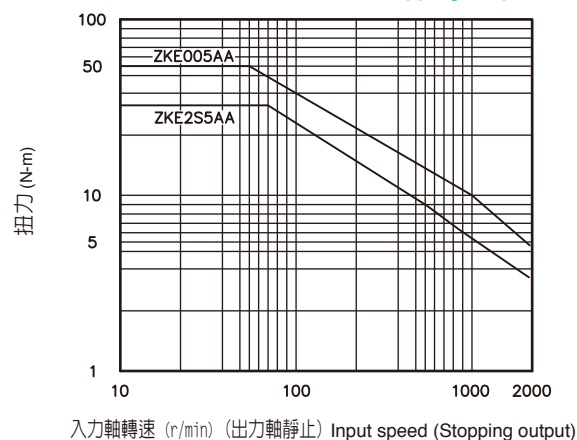
【容許滑動扭力特性圖】Allowable slipping torque chart
