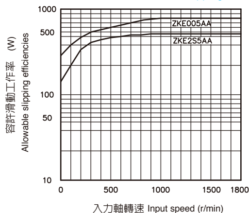
【容許滑動功率特性圖】Allowable slipping efficiency chart
