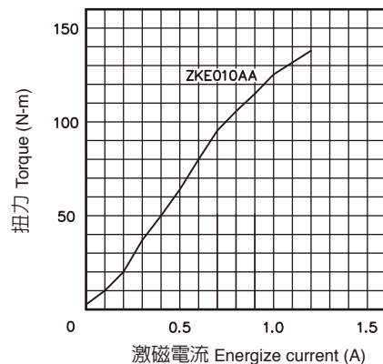
【容許滑動扭力特性圖】Allowable slipping torque chart
